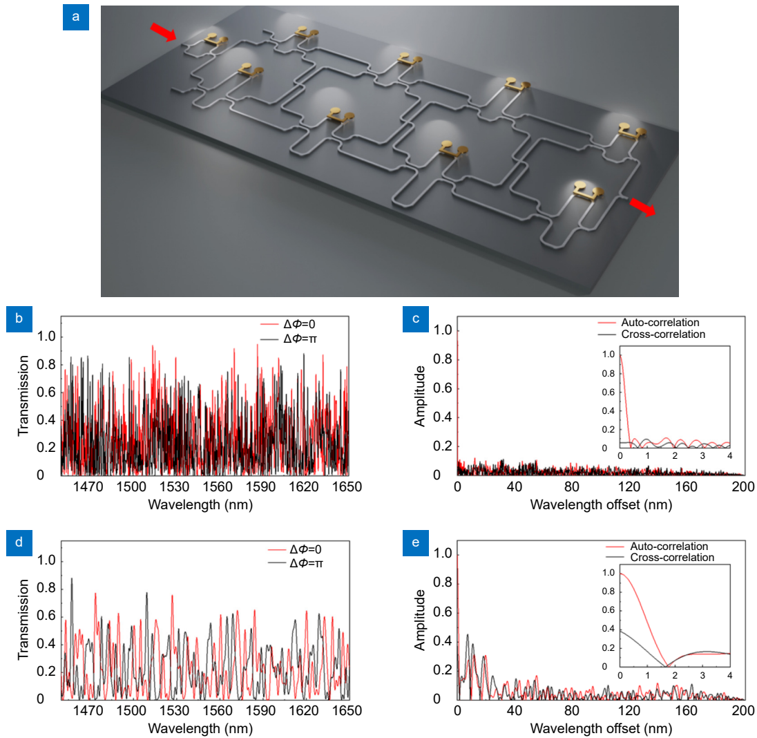
Fig. 2 | (a) Structure of our proposed programmable circuit. (b) Simulated spectral responses for the inversely designed structure with 0 and \pi phase changes applied to the 11 phase shifters, respectively. (c) Auto-correlation and cross-correlations of the spectral responses of the inversely designed circuit. (d) Simulated spectral responses for the randomly designed structure with 0 and \pi phase changes applied to the 11 phase shifters, respectively. (e) Auto-correlation and cross-correlations of the spectral responses of the randomly designed circuit.
