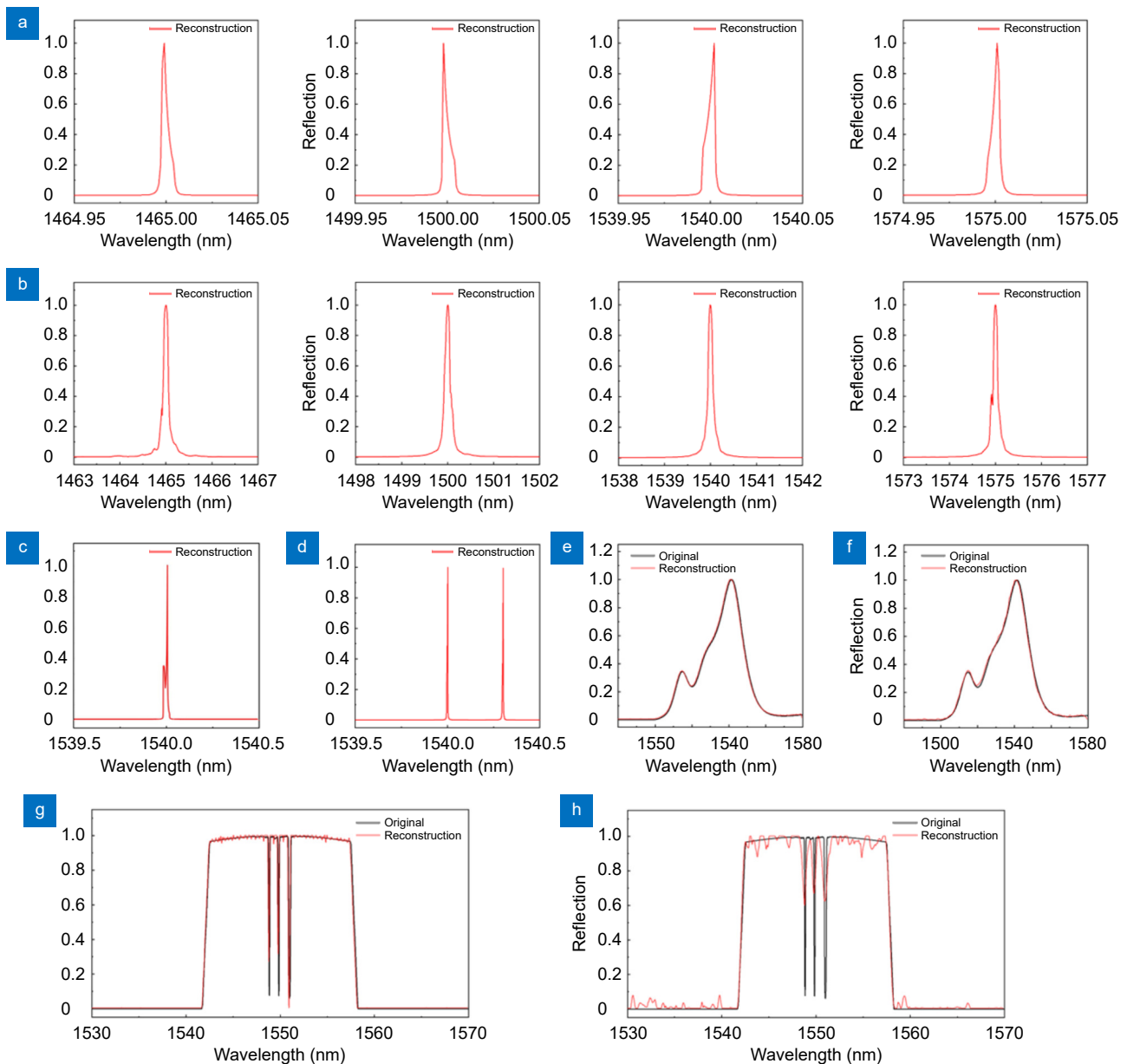
Fig. 6 | Reconstructions of various narrow peaks when the spectrometer working at mode 1(a) and mode 2(b), with a resolution of 6 pm and 150 pm, respectively. Reconstructions of two closely standing narrow peaks when the spectrometer working at mode 1(c) and mode 2(d), with a minimum distance of 15 pm and 300 pm, respectively. Reconstructions of broad spectrum when the spectrometer working at mode 1(e) and mode 2(f). Reconstructions of a complex dense spectrum when the spectrometer working at mode 1(g) and mode 2(h).
