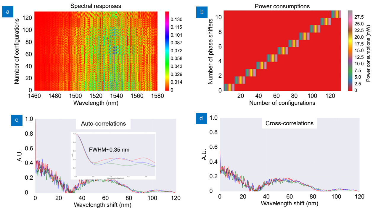
Fig. 5 | Experimental results when actuating 1 phase shifter at a time. (a) Spectral responses under 132 different configurations of all 11 phase shifters. (b) Power consumptions of the 11 phase shifters. (c) Exemplar auto-correlations of those spectral responses. (d) Exemplar cross-correlations between several spectral responses.
