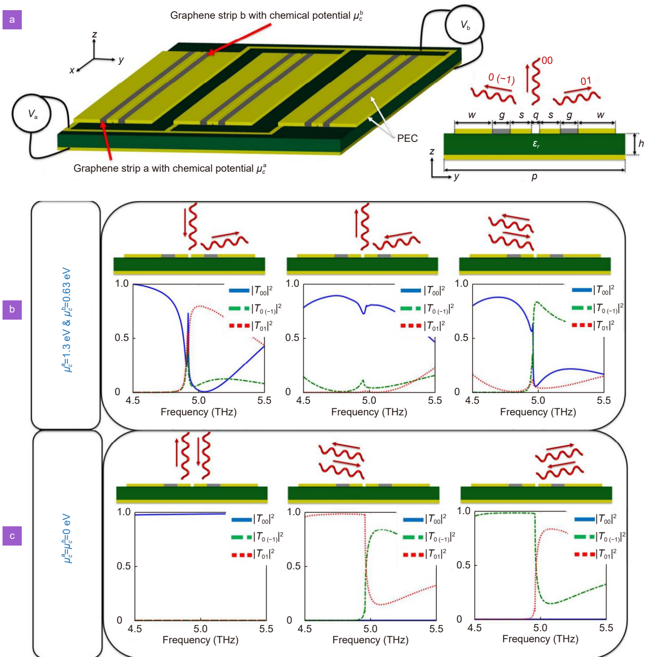
Fig. 9 | (a) Illustrative depiction of graphene based reconfigurable metagrating. Results for two different cases where (b) \mu_c^a = 1.3 eV and \mu_c^b = 0.63 eV, (c) \mu_c^a = \mu_c^b = 0 eV with design parameters p = 60.926 \mu\text{m} , w = 19.4 \mu\text{m} , s = 5 \mu\text{m} , g = 2.9 \mu\text{m} , h = 8.5 \mu\text{m} , q = 0.05 \mu\text{m} . Here the blue, green and red lines represents the transmittance for 00, 0(-1) or 0(1) diffraction modes respectively. Figures reproduced from: ref. 134 , American Chemical Society.
