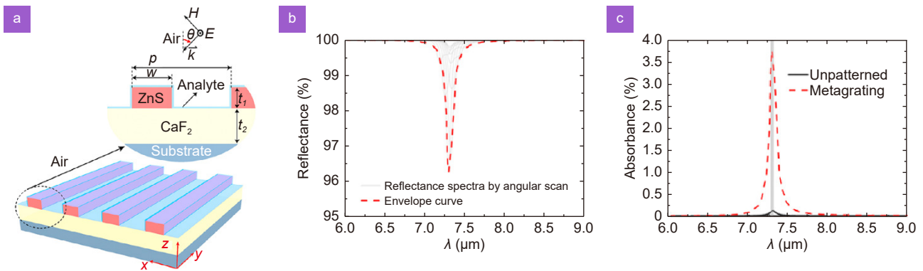
Fig. 12 | (a) Schematic representation of angle multiplexed metagrating. (b) A sequence of reflectance spectra obtained through angular scanning ranging from 16° to 25°, alongside their associated envelope curve, are presented for the metagrating coated with hBN. (c) The absorbance envelope curve and the reference absorbance spectrum of hBN. Figures reproduced with permission from: ref. 131 , De Gruyter, under the Creative Commons Attribution 4.0 International License.
