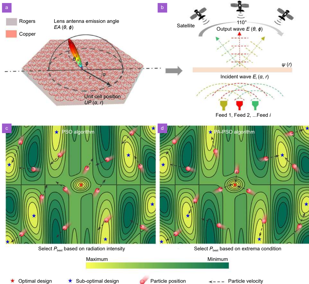
Fig. 1 | Schematics of the PA-PSO algorithm. (a) and (b) Working principle of the metalens antenna. (c) and (d) Comparison between the traditional PSO and PA-PSO algorithm. The red and blue stars represent optimal and sub-optimal designs, respectively. The red dots and dashed arrows represent the positions and velocities of the particles, respectively. (c) The working principle of the PSO algorithm where the swarm of particles is guided by the radiation intensity. (d) The PA-PSO algorithm guides the swarm of particles based on the extrema condition of the radiation intensity, which shows the correct directions of the maximum radiation intensity. This approach guides the swarm of particles more efficiently, which reduces not only the computation time but also the likelihood of finding sub-optimal designs.
